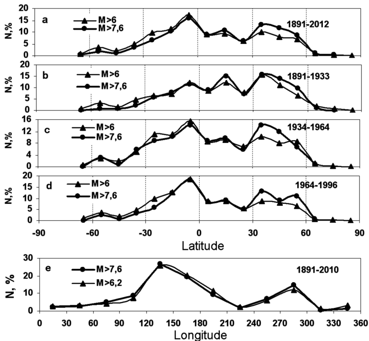
Figure 2. Latitudinal distribution of M \geq 6 and M \geq 7.6 earthquakes with a step size of 100 in a centennial cycle for the period 1891–2012: a – as a whole; b – for the initial period (1891–1933); c – for the average period (1934–1964); d – for the concluding period of a centennial cycle (1964–1996); e – longitudinal distribution of earthquakes with a step size of 300 in a centennial cycle for the above-mentioned period. The ordinate scale is expressed in percentages from the general number of earthquakes for the above-mentioned period.
