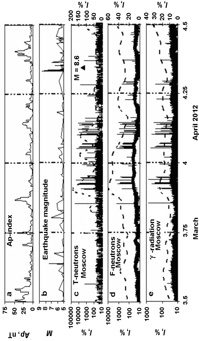
Figure 5. Temporal variations in March–April 2012: a – A_p index; b – earthquake magnitude ( M ); c–e – thermal and fast neutron and gamma radiation flux intensity, recorded at IZMIRAN, Moscow. The data on neutrons and gamma rays are in minutes (solid line, left-hand side scale) and in average daily values (dashed line, right-hand side scale).
