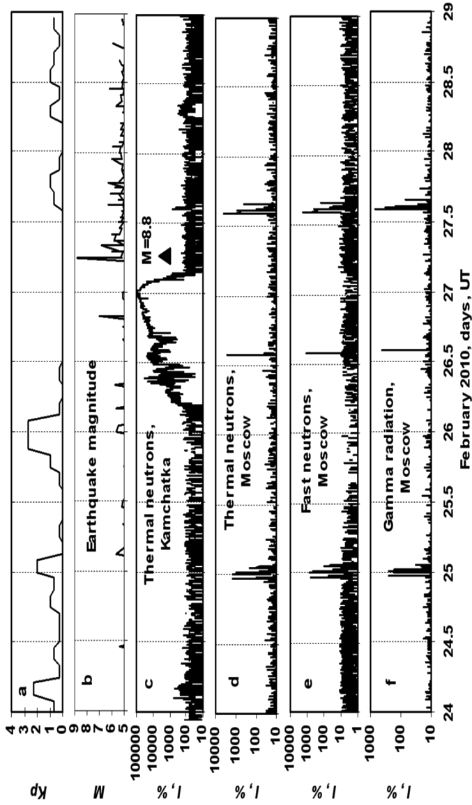
Figure 3. Temporal variations on February 24–29: a – Kp index; b – earthquake magnitude ( M ), c – thermal neutron flux intensity, recorded at the station in Kamchatka, d–f – thermal and fast neutron and gamma radiation flux intensity, recorded in Moscow.
